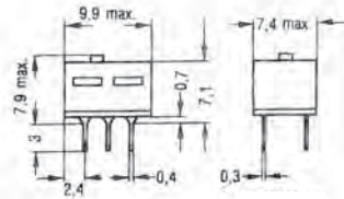
2 changeover contacts
